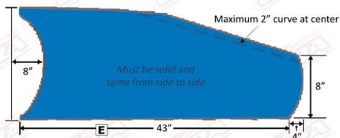
Spoiler Braces
