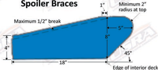
Spoiler Braces
